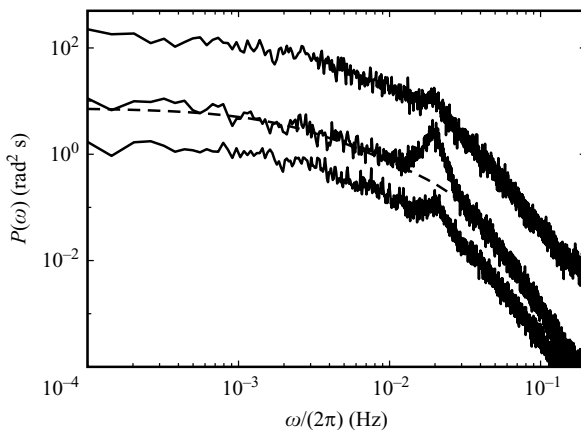
FIGURE 6. The solid lines denotes the power spectra P(\omega) of the slosh amplitude at Ra = 1.1 \times 10^{10} at the three vertical positions. Results for the top (bottom) row of thermistors at z = L/4 ( z = -L/4 ) were multiplied (divided) by a factor of 10 in order to make all three data sets distinguishable from each other. The dashed line denotes a fit of the predicted power spectrum for the background from (4.9) to the midplane ( z = 0 ) data.
