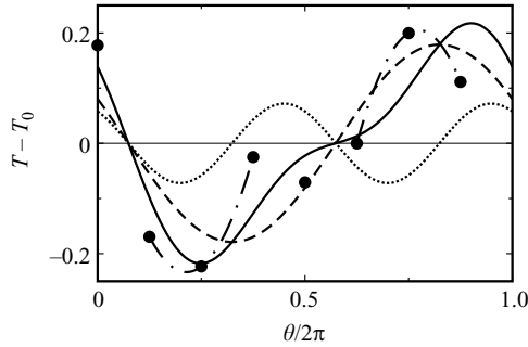
FIGURE 2. Example of a temperature profile measured by the sidewall thermistors at the midplane for R = 1.1 \times 10^{10} . The thin dash-dotted lines denote the TEE fit of extrema; the dashed line denotes cosine fit of (2.1); the dotted line denotes second-order sinusoidal term A_2 obtained from fitting (2.2) to the difference between the data and the cosine fit; the thick solid line denotes the fit obtained from the Fourier-moment method, corresponding to the sum of the dashed and dotted lines.
