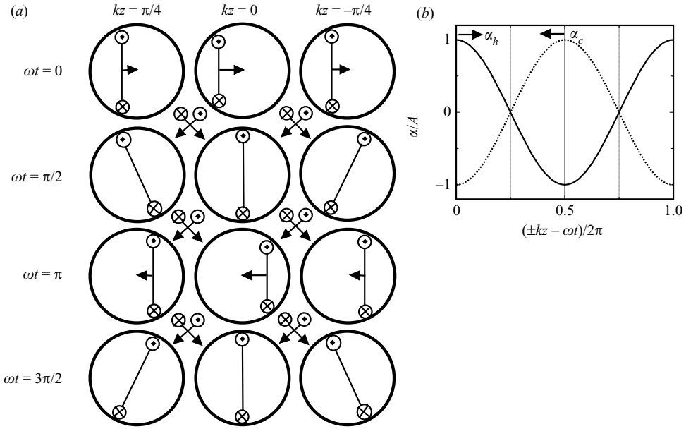
FIGURE 8. (a) The torsional and sloshing oscillations at different heights and phases in the Eulerian frame. Circled dot denotes \alpha_h where the LSC flow is upward. Circled cross denotes \alpha_c where the LSC flow is downward. Connecting lines denote the local plane of the LSC. Arrows pointing horizontally from the LSC plane denote restoring force on the LSC plane due to sidewall pressure. Arrows between diagrams indicate the viewing order to follow the advection of upward- and downward-moving plumes. Slosh displacements are seen at 2\omega_\phi t = 0, \pi , and twist displacements are seen at 2\omega_\phi t = \pi/2, 3\pi/2 . (b) Displacement angles of hot and cold plumes as functions of height and time. They can be seen as travelling waves moving in opposite directions. The +k is for \alpha_h moving to the right with increasing z , and the -k is for \alpha_c moving to the left with increasing z .
