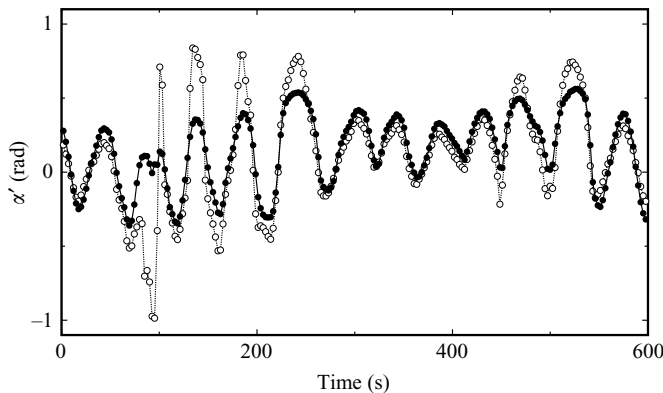
FIGURE 3. Time series of the slosh displacement angle \alpha' = (\alpha_h - \alpha_c)/2 for the middle-row thermistors at R = 1.1 \times 10^{10} : solid circles, from the Fourier-moment method; open circles, from the TEE method of Zhou et al. (2009).
