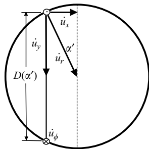
FIGURE 7. A horizontal cross-section showing the sidewall forcing for a horizontal displacement of the LSC. The solid vertical line corresponds to the plane of the LSC when it is displaced from a central alignment by the slosh displacement angle \alpha' . The component \dot{u}_y of the normal force F provides the centripetal acceleration for the LSC, and the component \dot{u}_x acts as the restoring force for a sloshing oscillation. The primary LSC velocity u_\phi is perpendicular to this cross-section.
